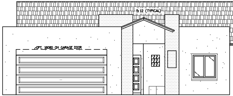
FRONT ELEVATION - GABLE ENTRY
