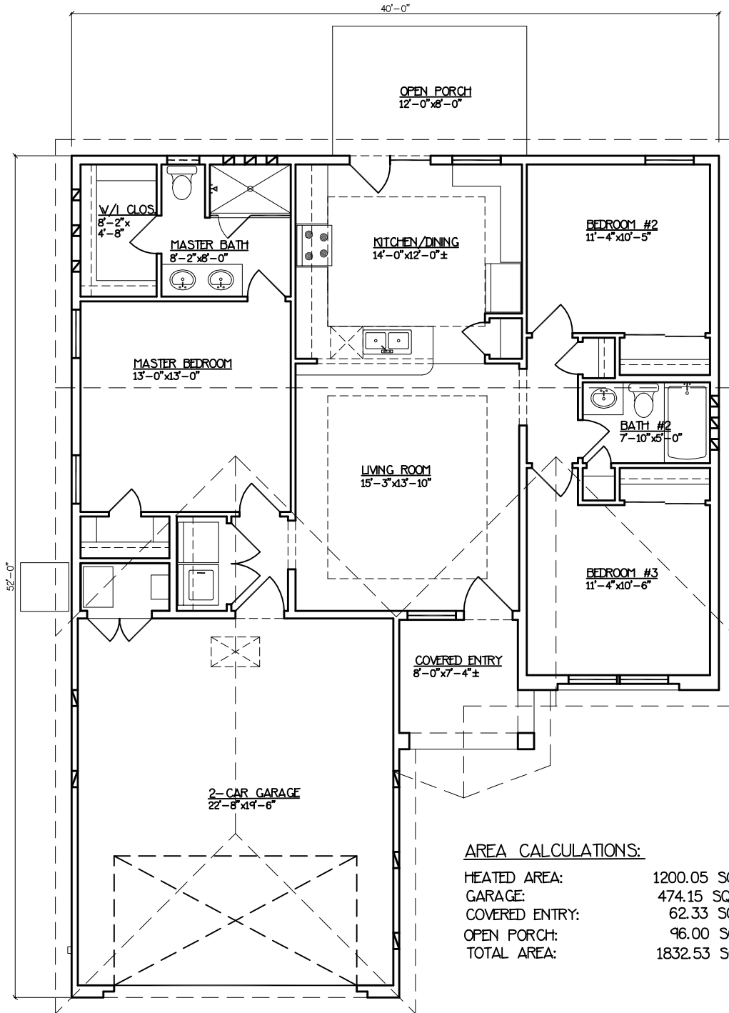
FLOOR PLAN
